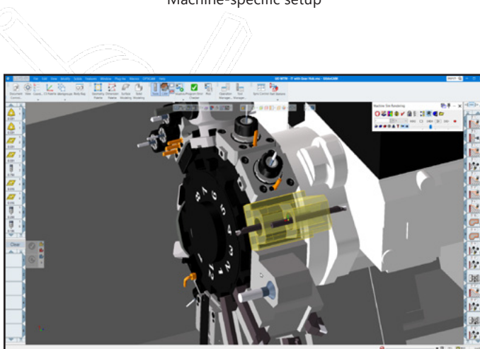
Intermediate tooling provides more accurate simulation of cutting motion
